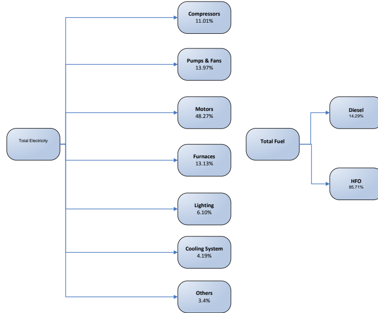
Figure 12: Energy End-Use Model of the packing, packaging, paper, cartoon and stationeries sector.
