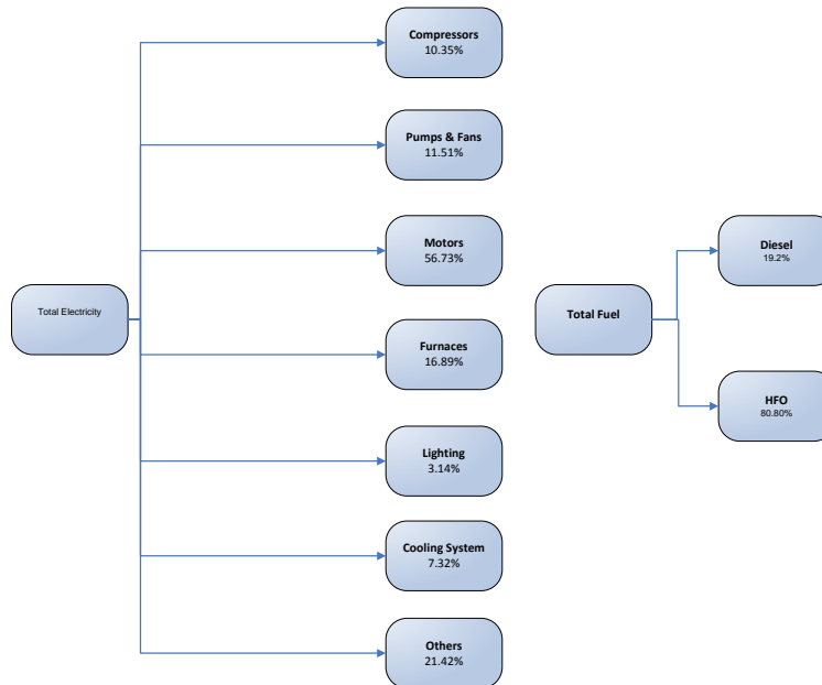
Figure 13: Energy End-Use Model of the mining sector.
