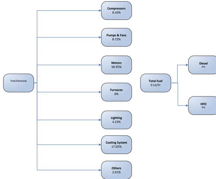
Figure 7: Energy End-Use Model of the plastic and rubber sector.
