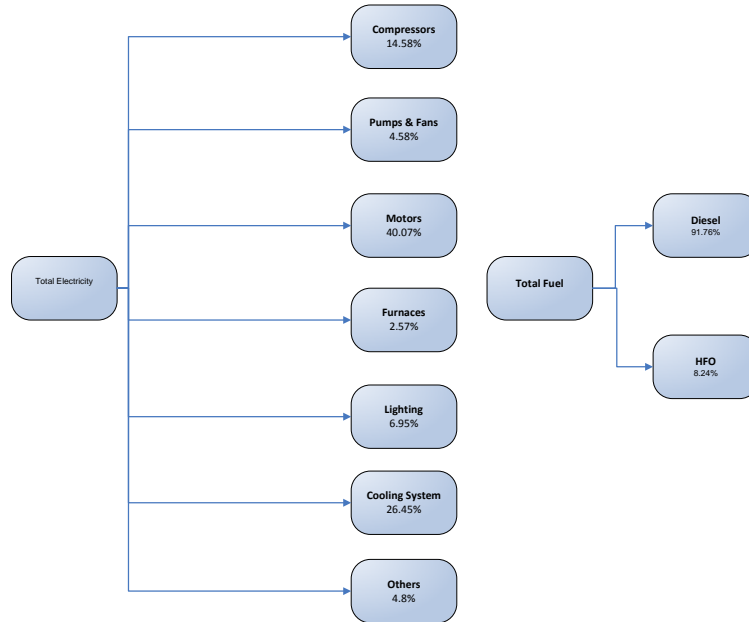
Figure 11: Energy End-Use Model of the food, supplies, agriculture and livestock sector.
