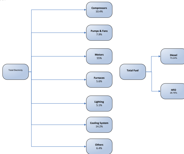
Figure 3: Energy End-Use Model of the Jordanian SMEs Industries.
