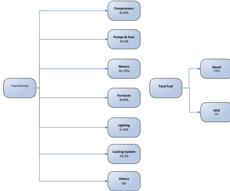
Figure 8: Energy End-Use Model of the engineering, electrical industries and information technology sector.
